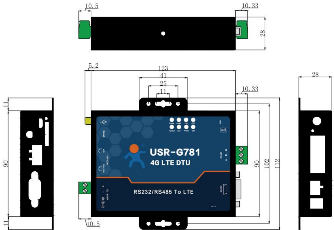
USR-G781 Dimensions
