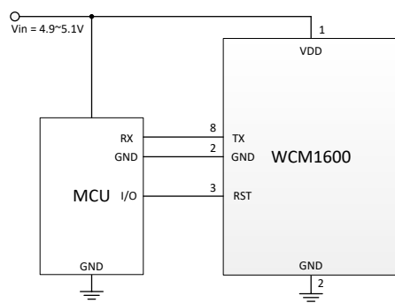
APP. 1. Output UART signal with MCU
