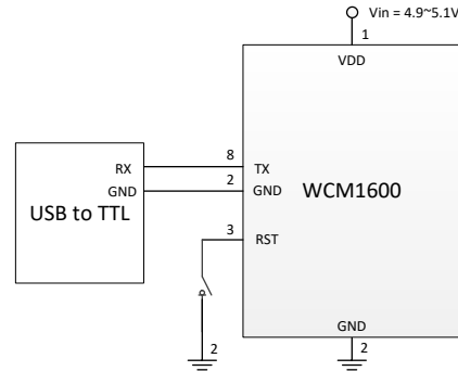
APP. 2. Output UART signal with USB to TTL
