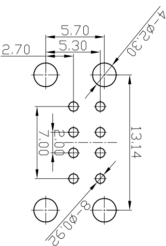
P. C. B LAYOUT (对接尺寸)
